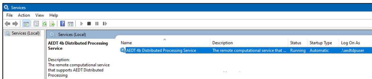
Figure 5-45 Services Dialog
