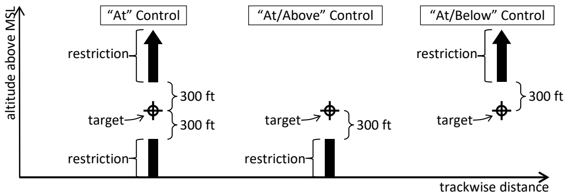
Figure 3-19 Altitude Controls
