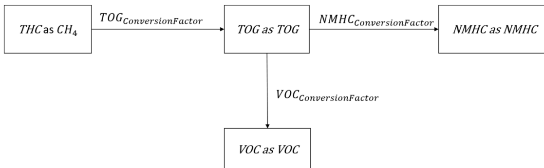
Figure 5-1 TOG, NMHC, and VOC Calculations for Turbine Engines
