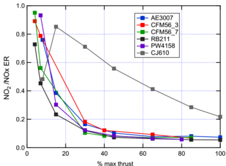
Figure 6-6 NO 2 /NO x Ratios for Jet Engines from Timko et. al
