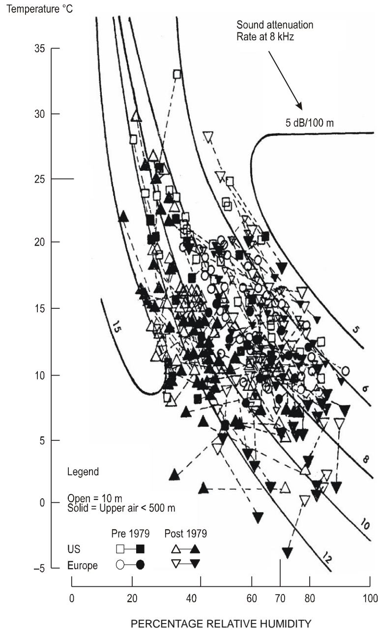
Figure 11-4 Meteorological Conditions Recorded During Noise Certification Tests 56
