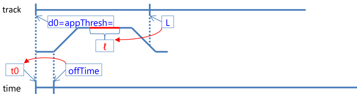
Figure 3-13 Track Alignment – Circuit Procedure
